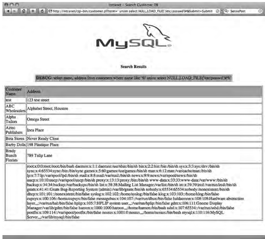
Figure 6.3 Reading /etc/passwd through the Database
