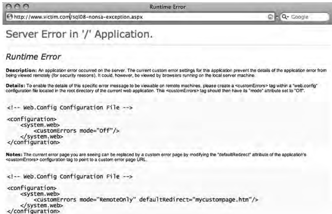
Figure 5.8 Default Exception Page in ASP.NET
