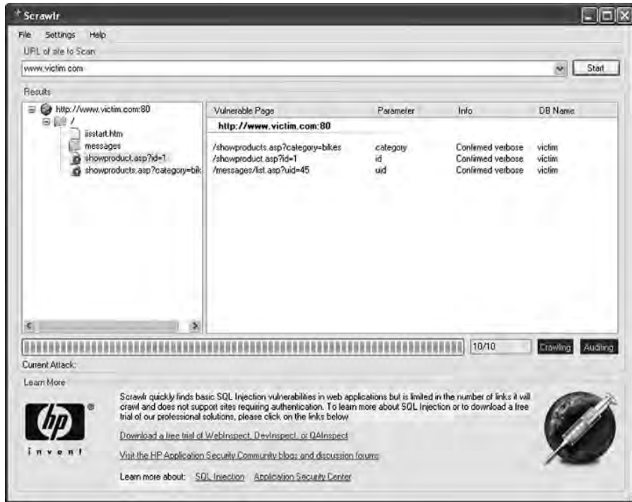
Figure 2.19 HP Scrawlr
