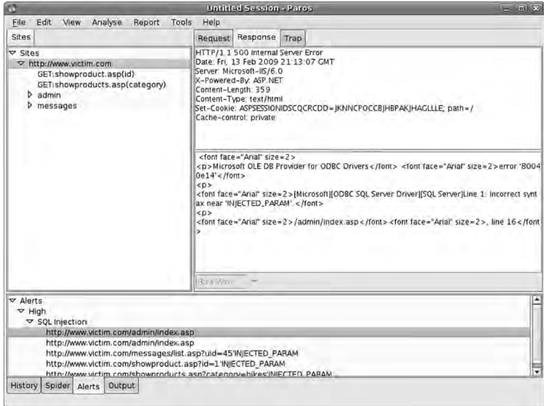
Figure 2.21 Paros Proxy
